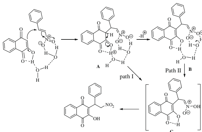
Scheme 2. Plausible mechanism for the formation of nitroalkylated 2-hydroxynaphthoquinone.
